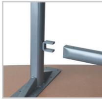
FOR LEARN-IT Flattened oval tube shape cross bar assembly with tamper resistant screws. Leg plate with welded angled supports attaches with metal inserts.
