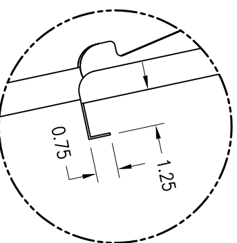
CHALK TRAY DETAIL
