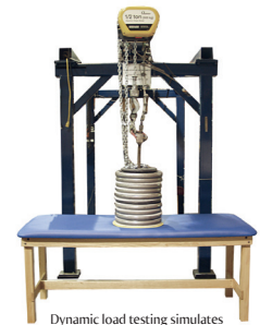
Dynamic load testing simulates real-life hop and drop table use.
